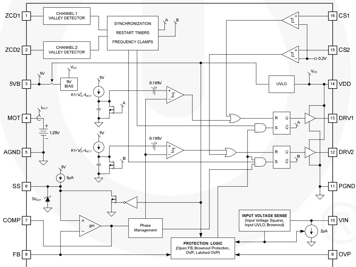
Figure 1. Block Diagram
