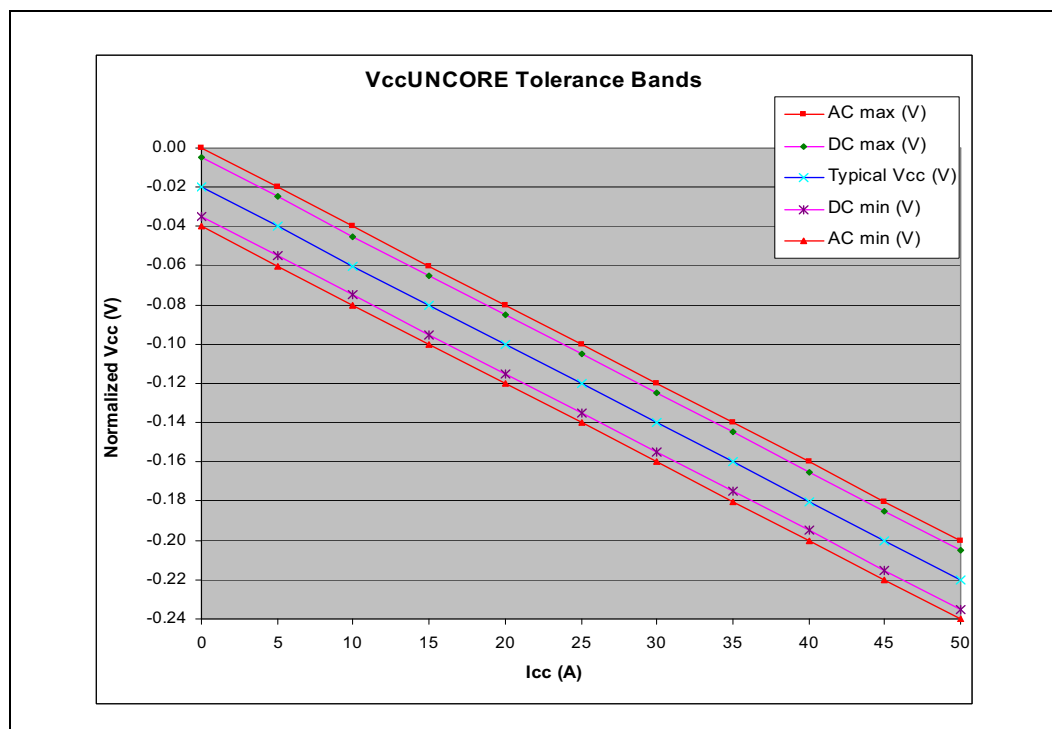
Figure 2-10. V_{CCUNCORE} Static and Transient Tolerance for Intel® Itanium® Processor 9300 Series
