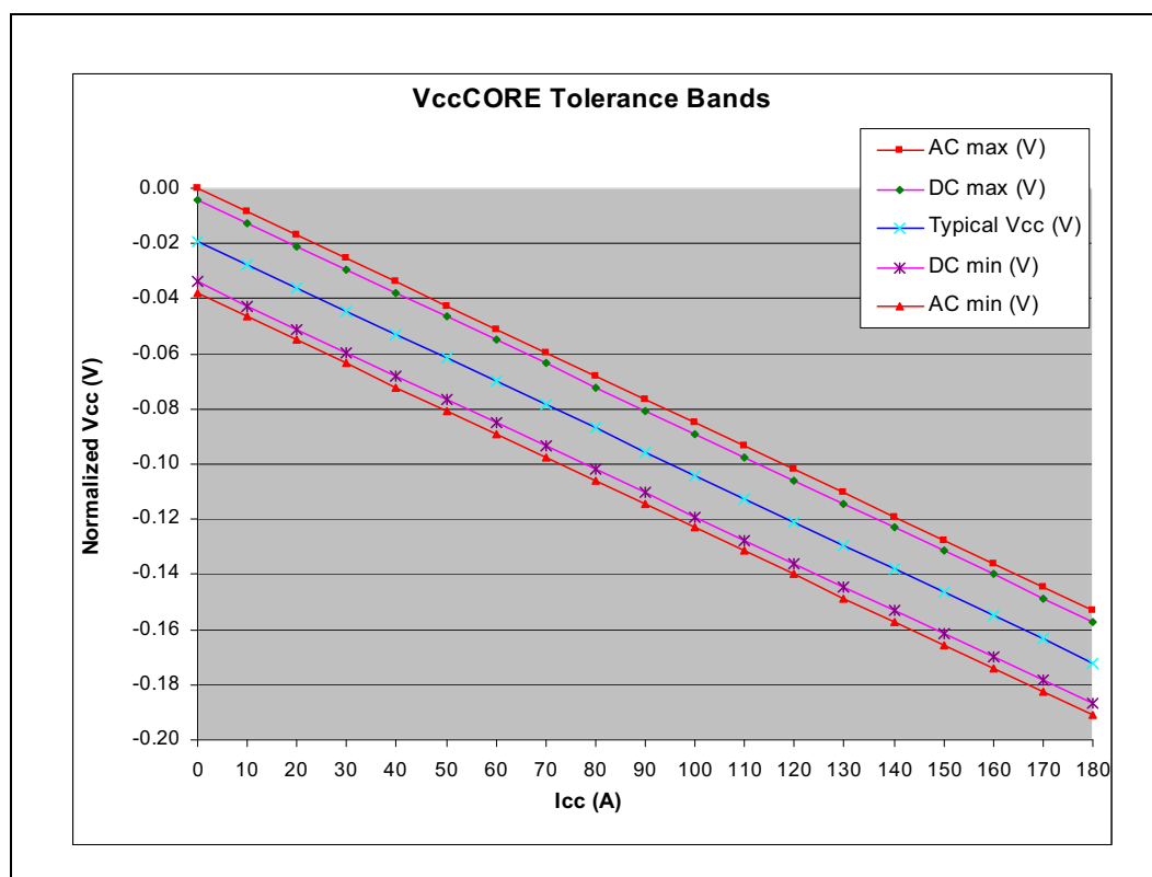
Figure 2-11. V CC CORE Static and Transient Tolerance for Intel® Itanium® Processor 9300 Series
