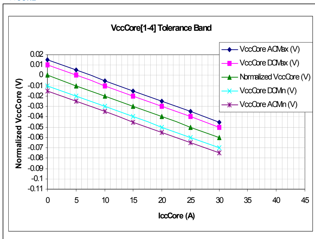
Figure 2-15. V CC CORE Load Line for the Intel® Itanium® Processor 9500 Series
