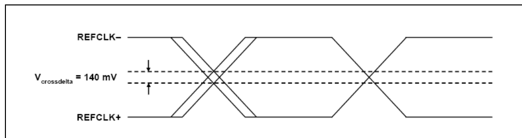
Figure 2-3. V_{\text{cross-delta}} Definition
