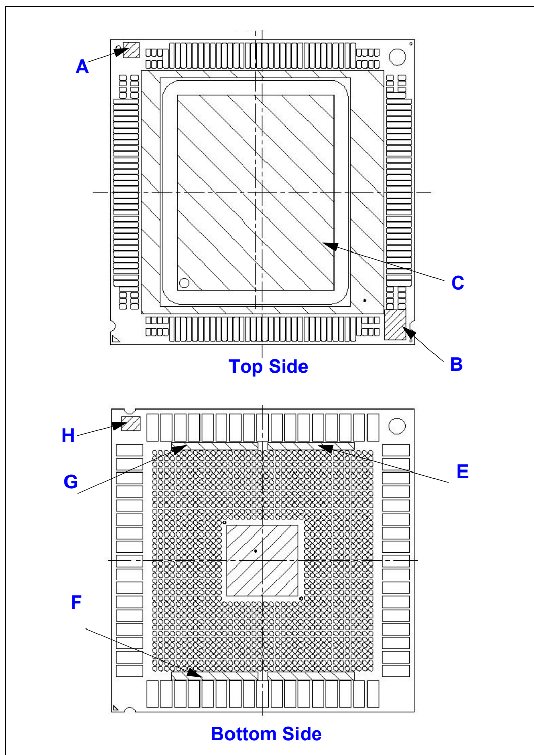
Figure 4-10. Processor Marking Zones
