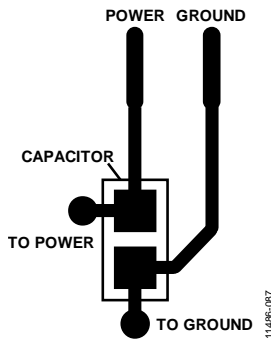
Figure 81. Recommended Power Supply Bypass Capacitor Layout
