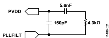
Figure 17. PLL Filter
