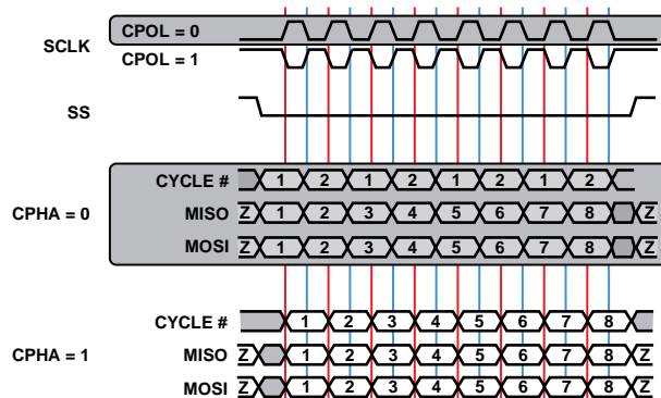
Figure 35. Clock Polarity and Phase for SPI Slave Port
