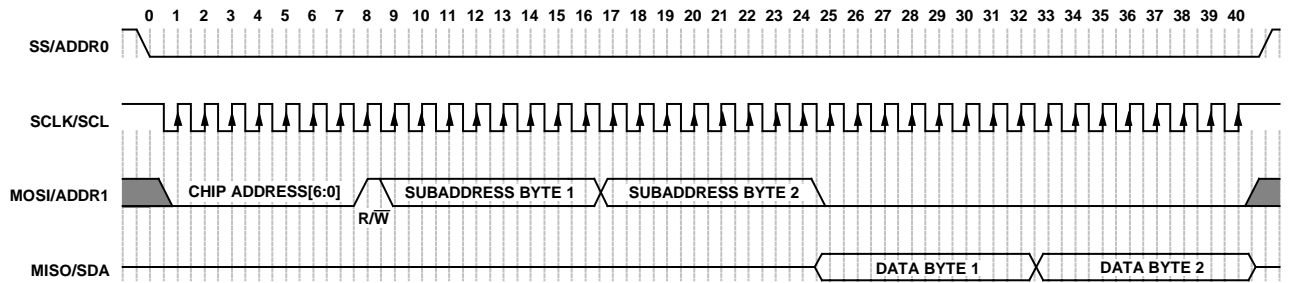
Figure 37. SPI Slave Read Clocking (Single Word Mode, Two Bytes)
