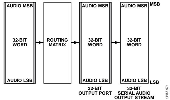
Figure 67. 32-Bit Serial Output Example
