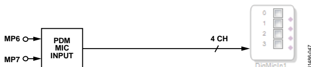
Figure 44. PDM Microphone Input Mapping to DSP in SigmaStudio
