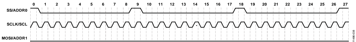
Figure 34. Example of SPI Slave Mode Initialization Sequence Using Dummy Writes
