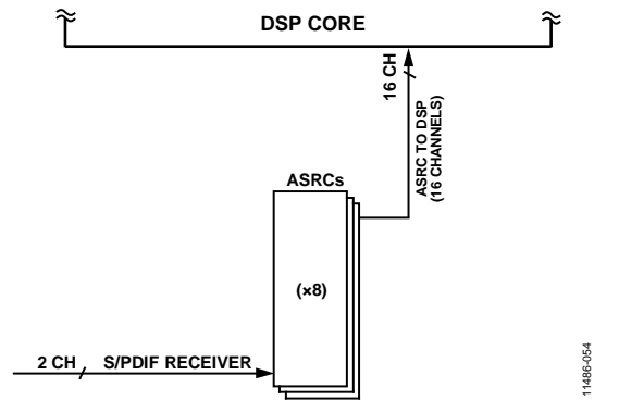
Figure 51. Example ASRC Routing for Asynchronous Input to the DSP Core
