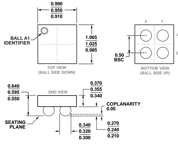
Figure 38. 4-Ball, Wafer Level Chip Scale Package [WLCSPP] (CB-4-4) Dimensions show in millimeters
