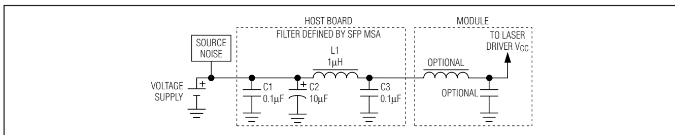
Figure 3. Supply Filter
