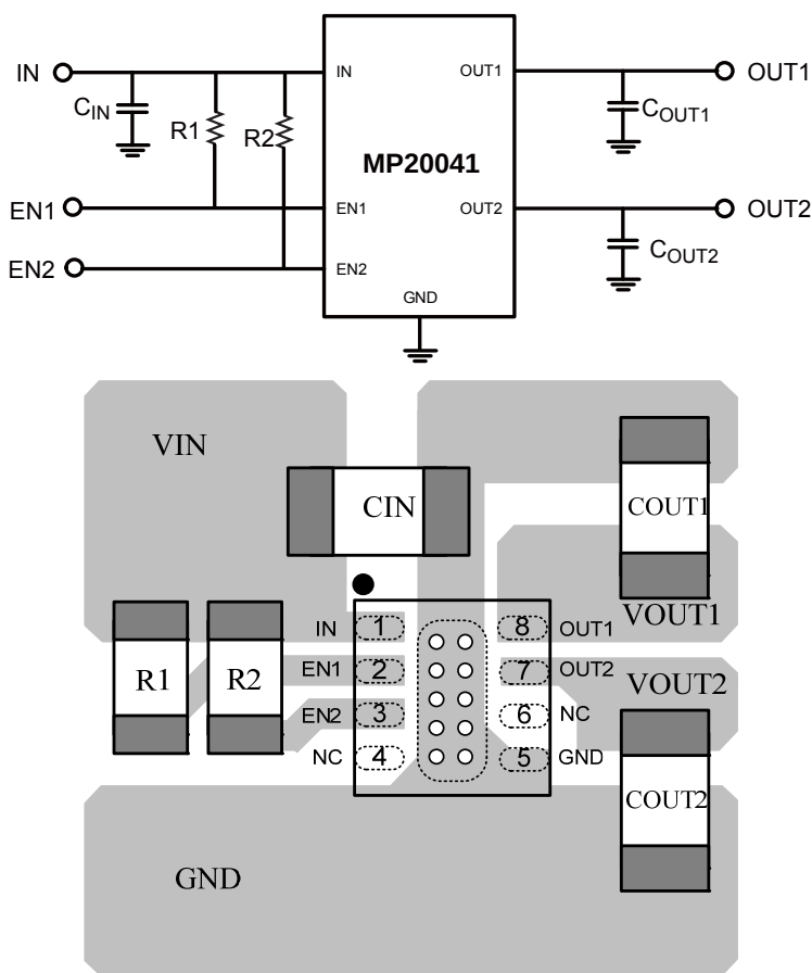
Top Layer Figure 5—PCB Layout
