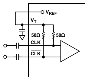
Figure 21. AC-Coupling Differential Signals Inputs, Such as LVDS
