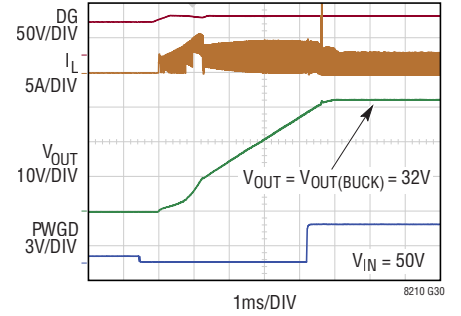
Pass-Thru Start-Up: V IN Above Pass-Thru Window (Figure 38)
