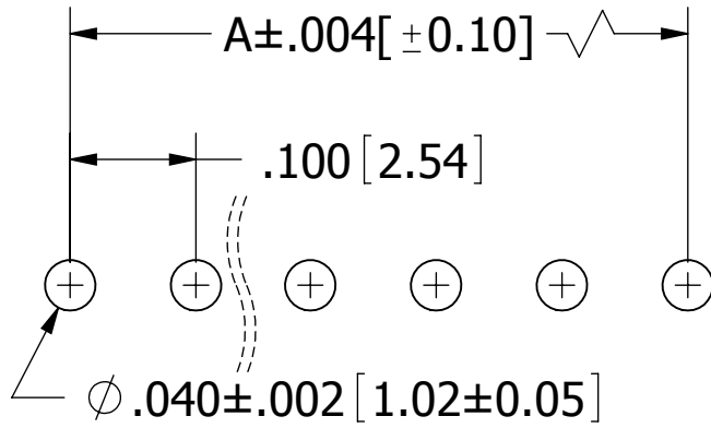
RECOMMENDED PCB LAYOUT SINGLE ROW TOLERANCE: ±.002 [±0.05]
