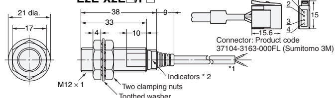
Diagram 9 E2E-X3D□ E2E-X2E□/F□ Pre-wired e-CON Connector Models 5.9 1
