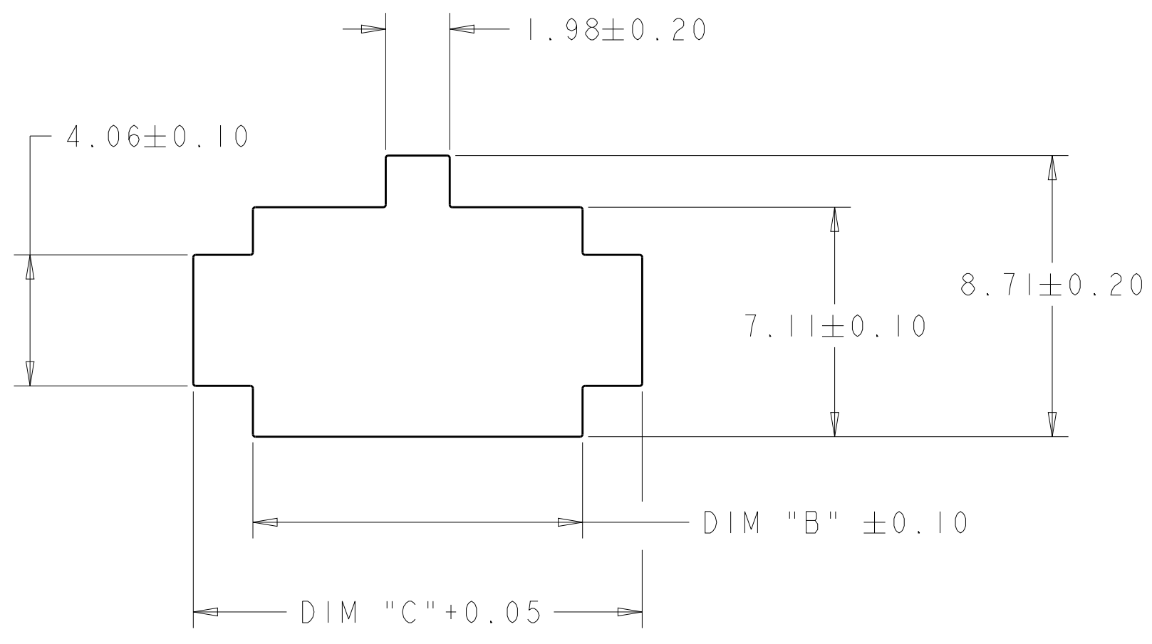
PANEL CUT-OUT 1
