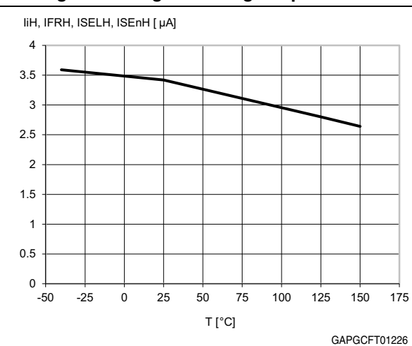
Figure 20. High level logic input current
