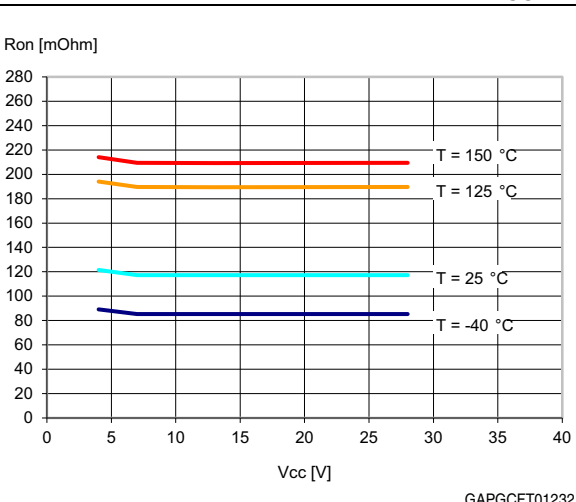
Figure 26. On-state resistance vs. V_{CC}
