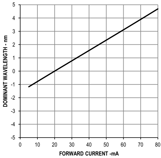
Figure 6: Wavelength vs. Forward Current
