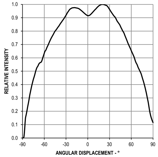
Figure 5: Intensity vs. Angle
