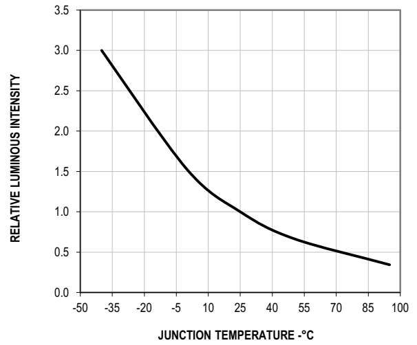
Figure 7: Intensity vs. Temperature
