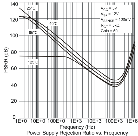
Power Supply Rejection Ratio vs. Frequency
