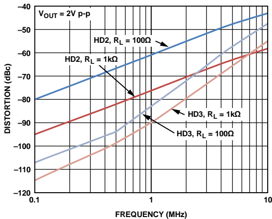
Figure 16. Harmonic Distortion vs. Frequency for Various Loads
