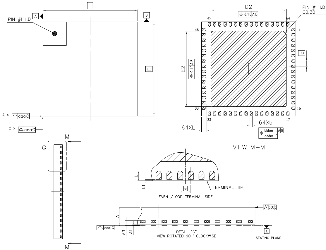
Figure 4.3. QFN64
