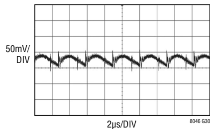
Output Ripple
