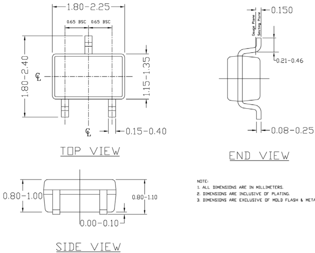
3-Pin SC-70 (C3)
