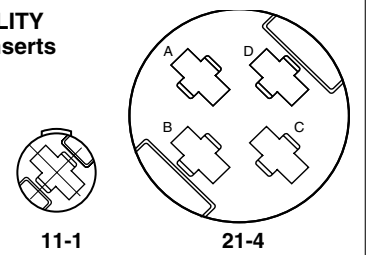
MT38999 Connectors
