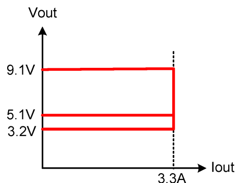
V/I Profile
