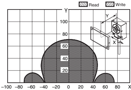
V680-HS63 (mounted on metallic material) & V680-D8KF68/-D32KF68 (mounted on metallic surface: steel) (Horizontal-facing RF Tag) When the V680-A81 attachment is mounted on RF Tag
