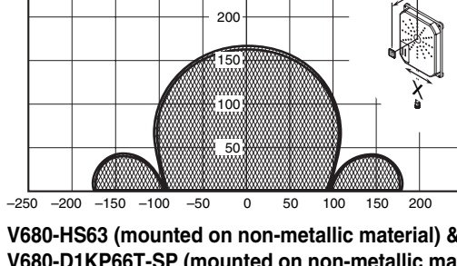
V680-H01-V2 (mounted on non-metallic material) & V680-D1KP66T (mounted on non-metallic material)
