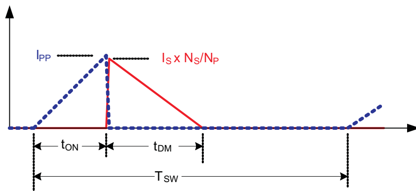
Figure 16. Transformer Currents
