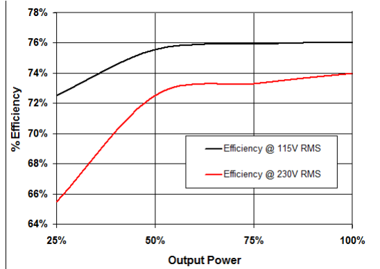
Figure 20. Efficiency
