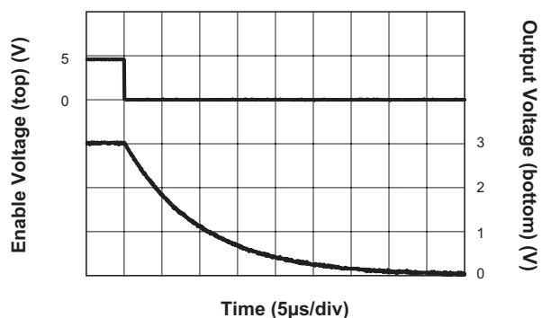
Turn-Off Response Time ( I_{OUT} = 100mA )
