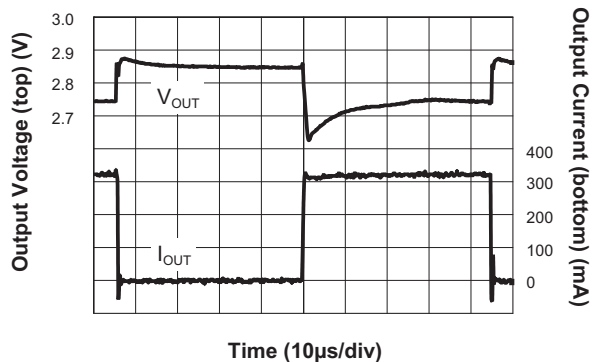
Load Transient Response 300mA ( V_{OUT} = 2.8V )
