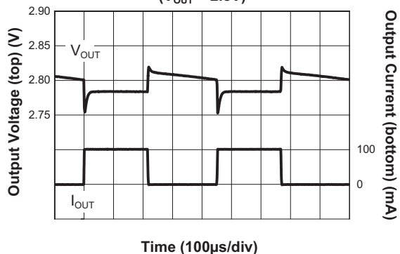
Load Transient Response ( V_{OUT} = 2.8V )
