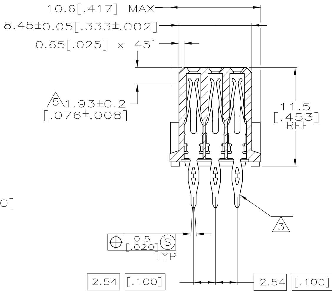
SECTION X-X
