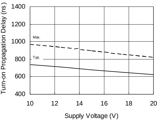
Figure 13B. Turn-On Propagation Delay Time vs. Supply Voltage
