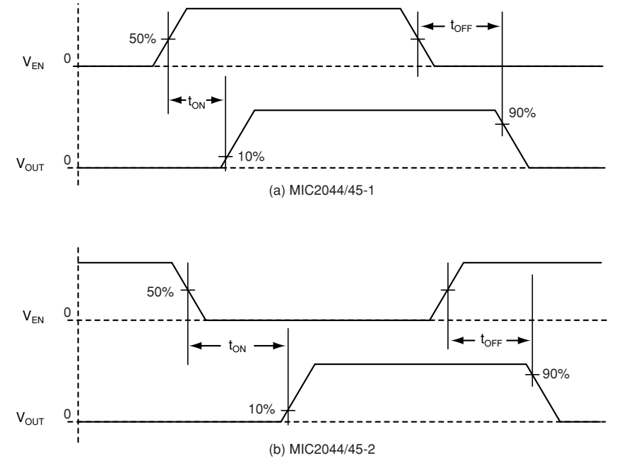
Figure 1. Turn-On/Turn-Off Delay
