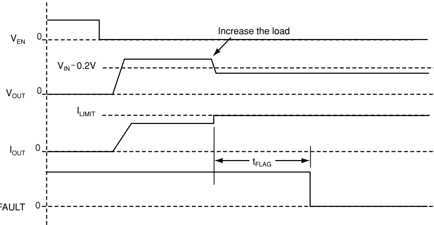
Figure 2. Overcurrent Fault Response — MIC2044-2
