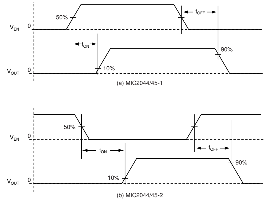
Figure 1. Turn-On/Turn-Off Delay
