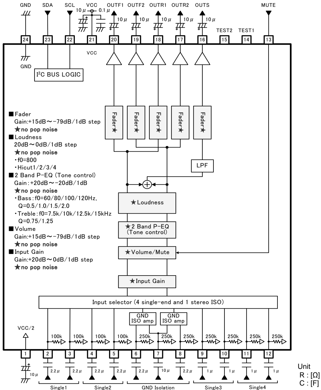
Fig. 22 BD37523FS
