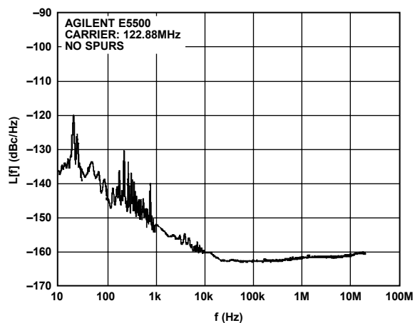
Figure 8. Phase Noise at 122.88 MHz
