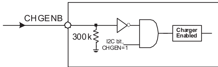
Figure 8. Charger enable
