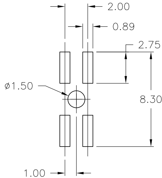
RECOMMENDED PCB LAYOUT 4 WAY CONNECTORS
