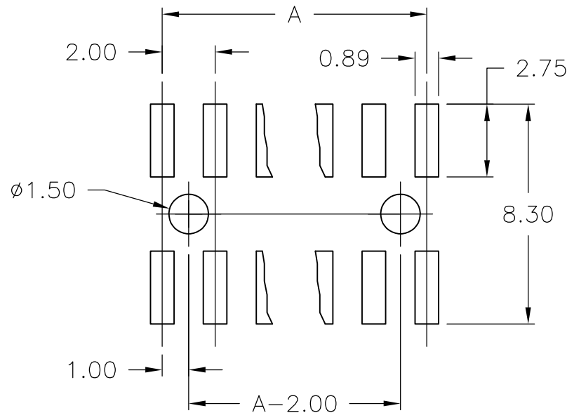
RECOMMENDED PCB LAYOUT 6 TO 20 WAY CONNECTORS
