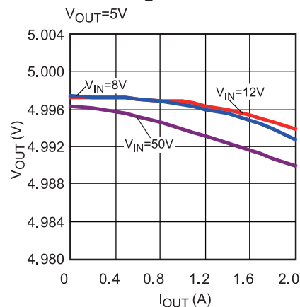
Load Regulation
