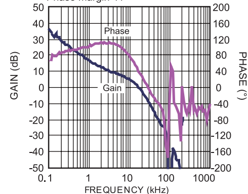
Loop Gain with Phase Margin
