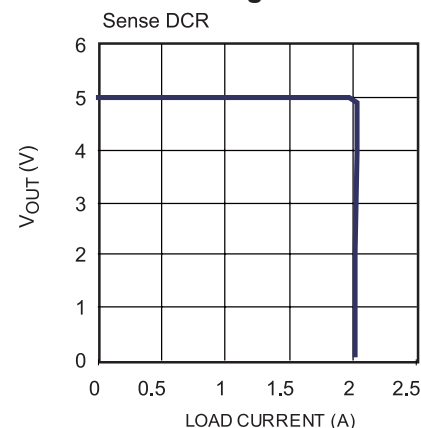
Current Regulation
