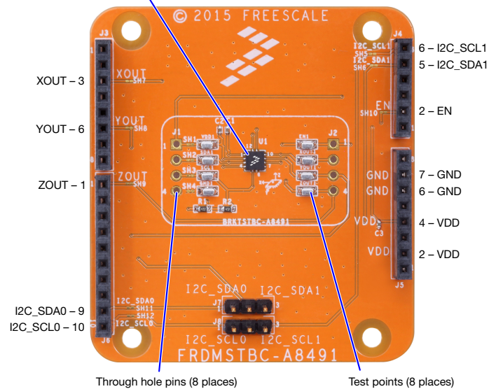
MMA8491Q 3-axis multifunction digital accelerometer 12 QFN (3 mm x 3 mm x 1.05 mm)
