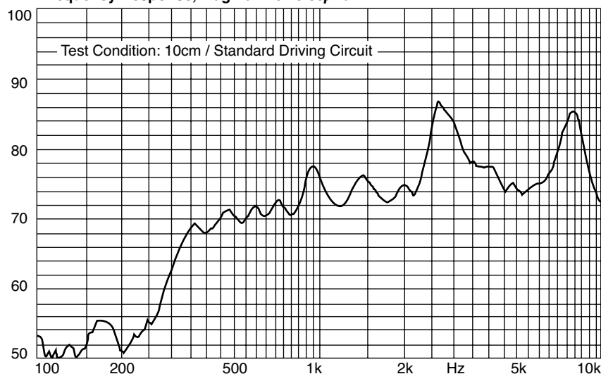
Frequency Response, Magn dB re 20.00μPa
