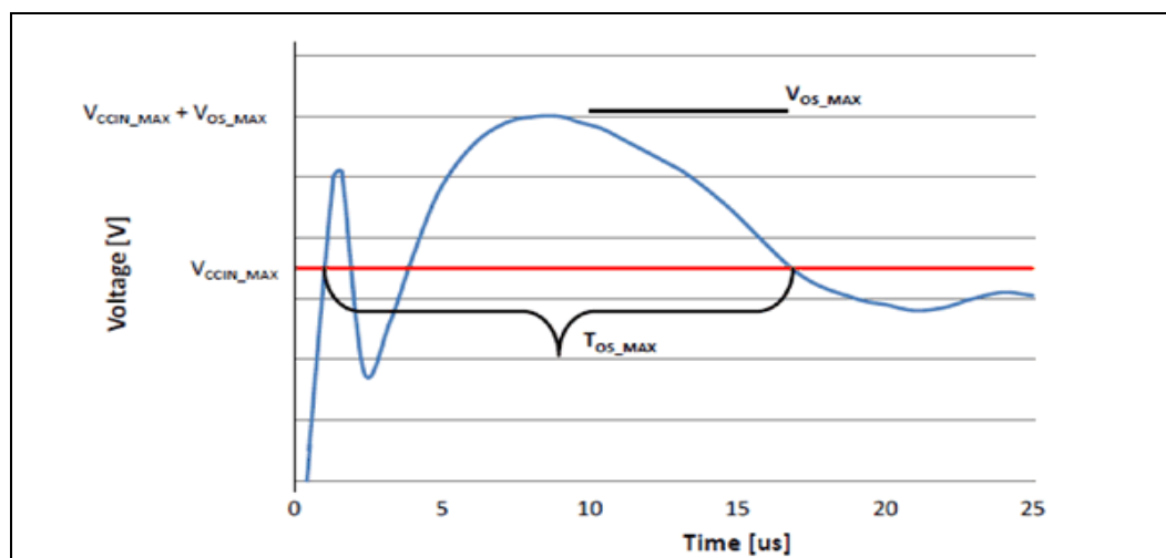
Figure 2-4. VCCIN Overshoot Example Waveform
