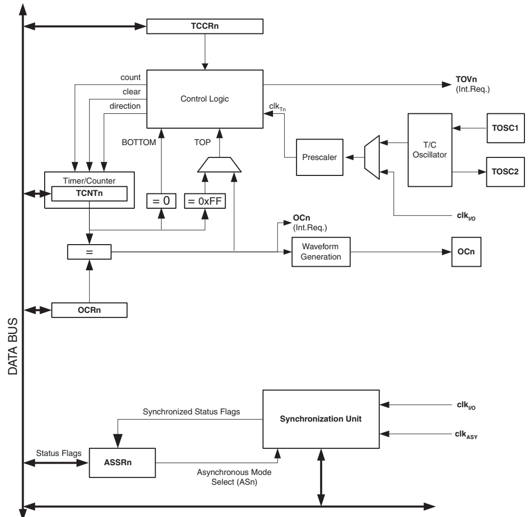
Figure 53. 8-bit Timer/Counter Block Diagram
