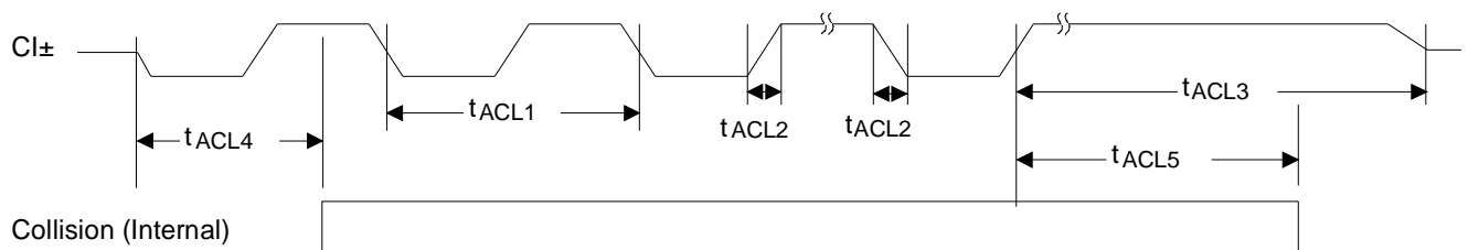
Figure 46. AUI Collision
