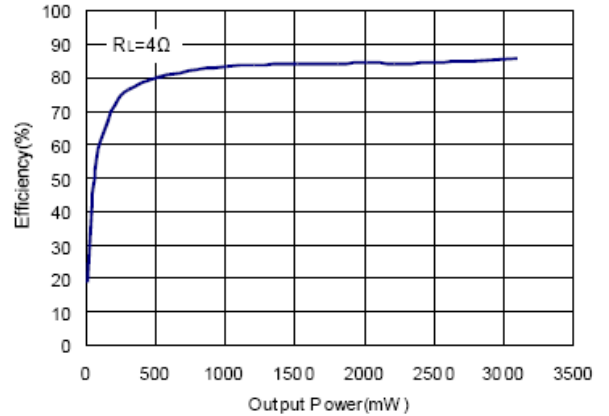
12. Efficiency VS Output Power
