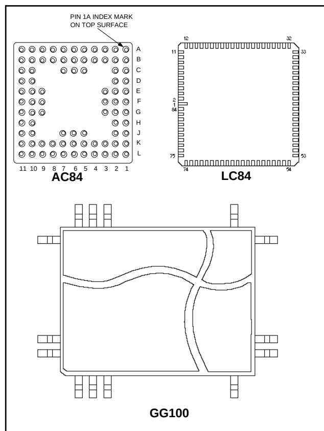
Fig.1 Pin connections - bottom view
