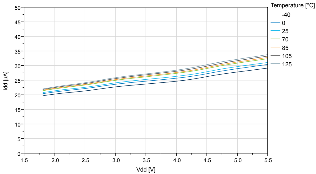
Figure 35-50. BOD Current vs. V_{DD} (Continuous Mode Enabled)
