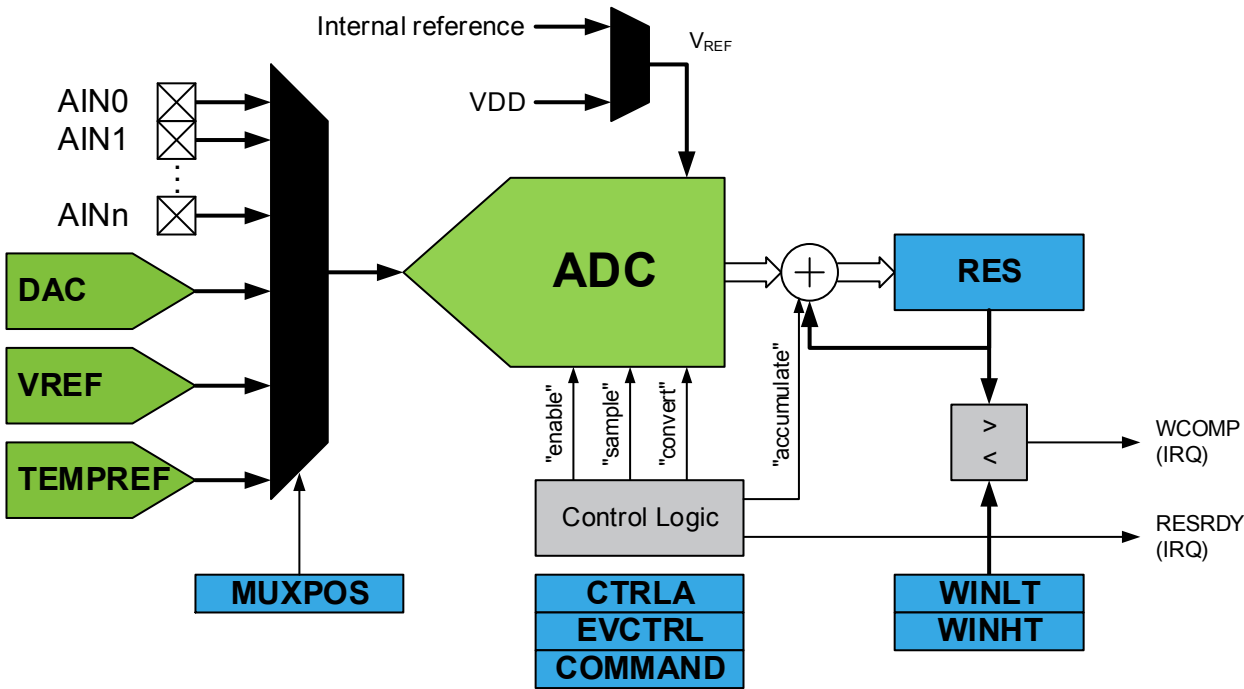
Figure 30-1. Block Diagram
