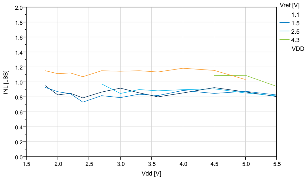
Figure 35-62. INL vs. V_{DD} (115ksps) at T=25^{\circ}C
