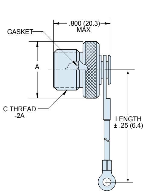
667-217 Plug Cover
