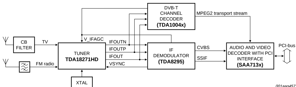
Fig 26. Example of hybrid reception for PCTV applications
