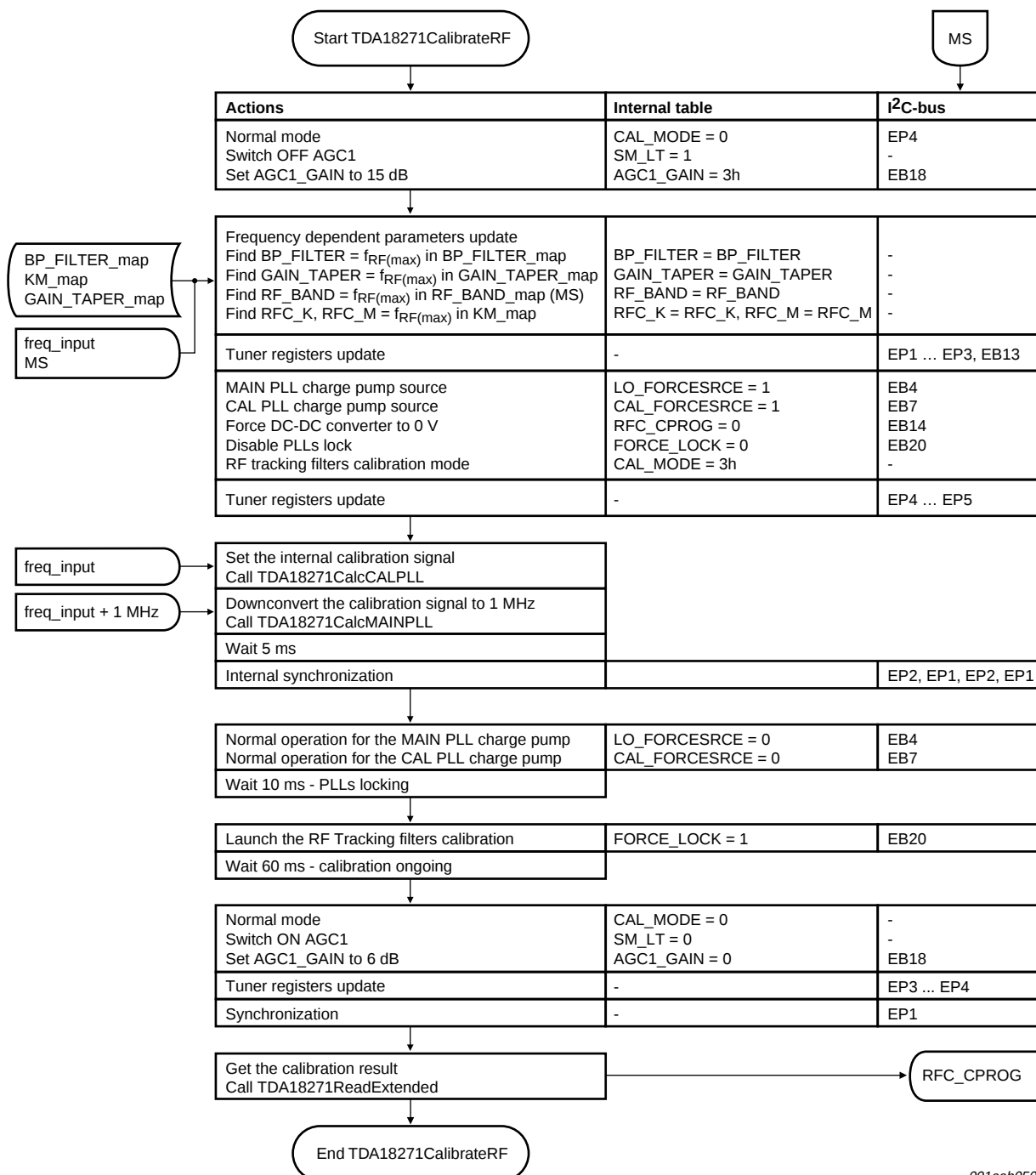
Fig 14. Flowchart TDA18271CalibrateRF
