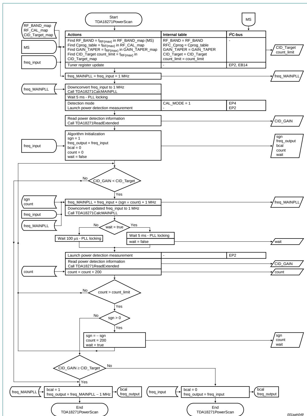
Fig 13. Flowchart TDA18271PowerScan
