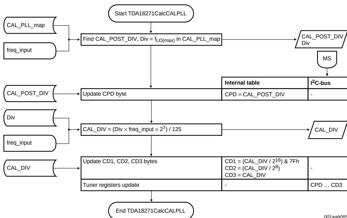
Fig 19. Flowchart TDA18271CalcCALPLL
