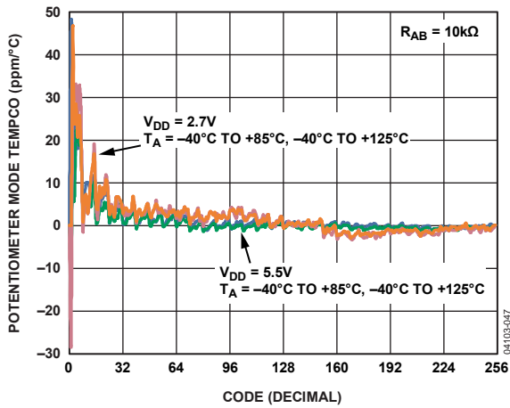
Figure 18. AD5172 Potentiometer Mode Tempco \Delta V_{WB}/\Delta T vs. Code
