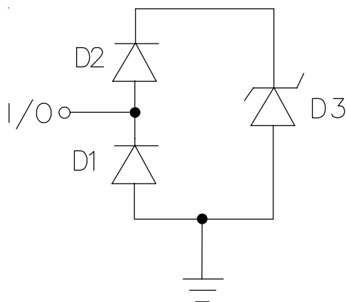
RClamp2504P Spice Model
