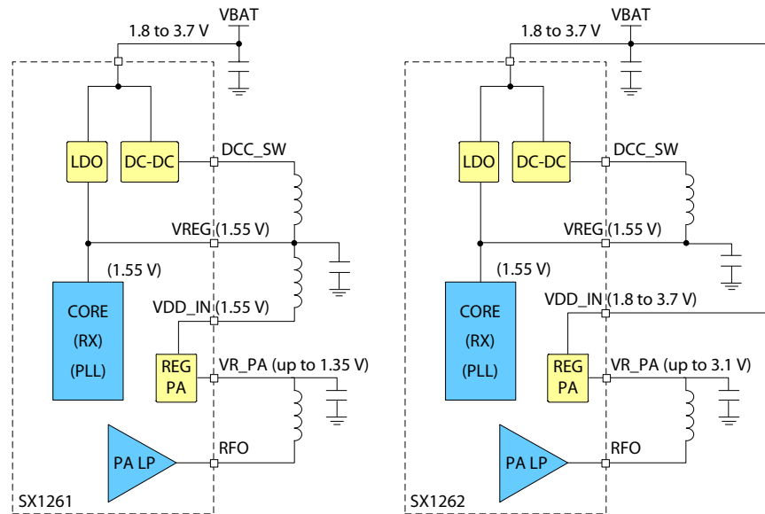
Figure 4-3: PA Supply Scheme in DC-DC Mode
