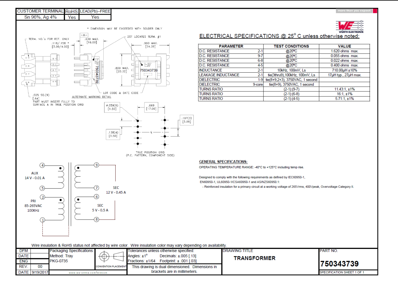
Figure 34 Transformer structure
